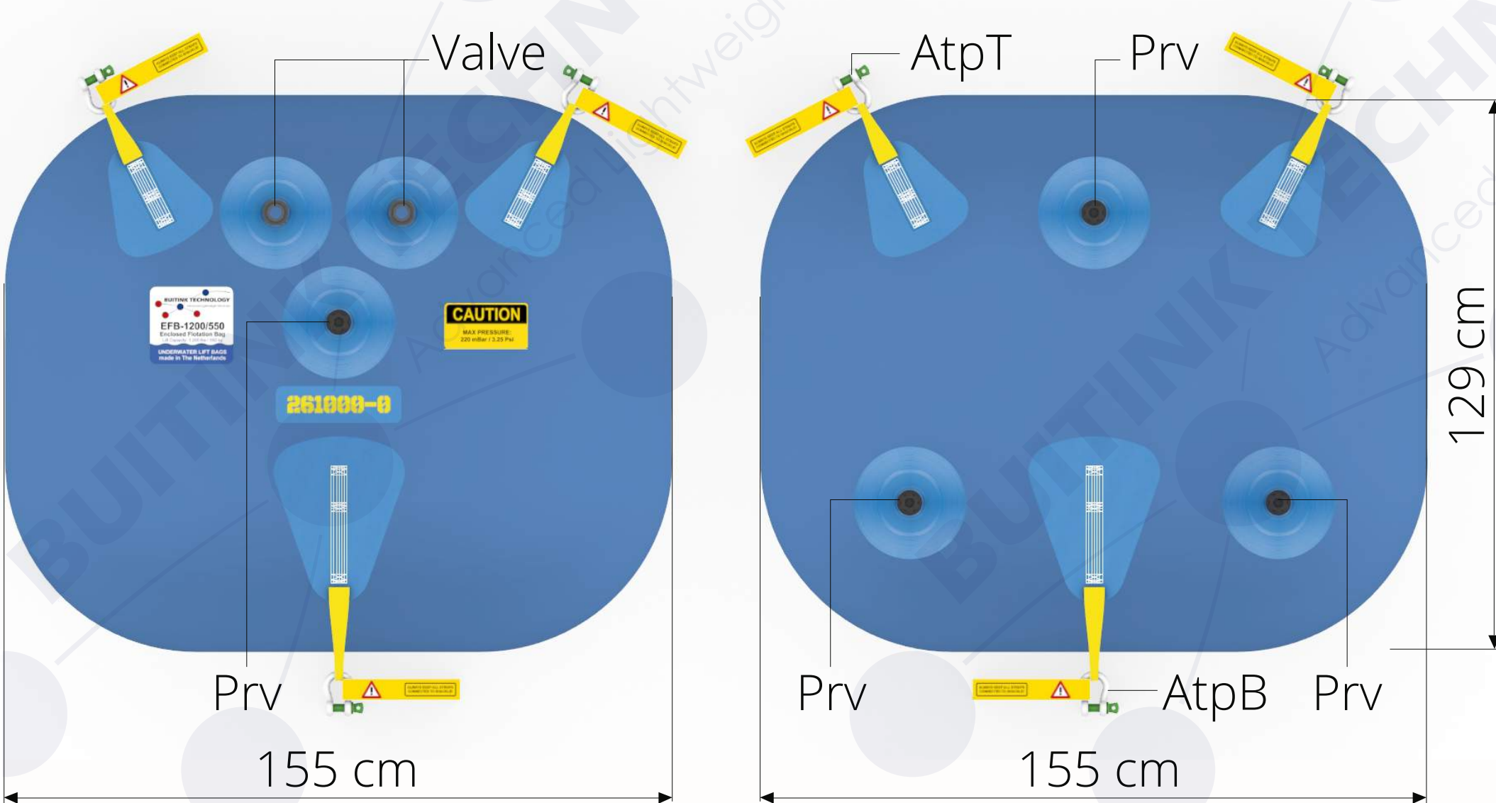
EFB-1200/550 FRONT
