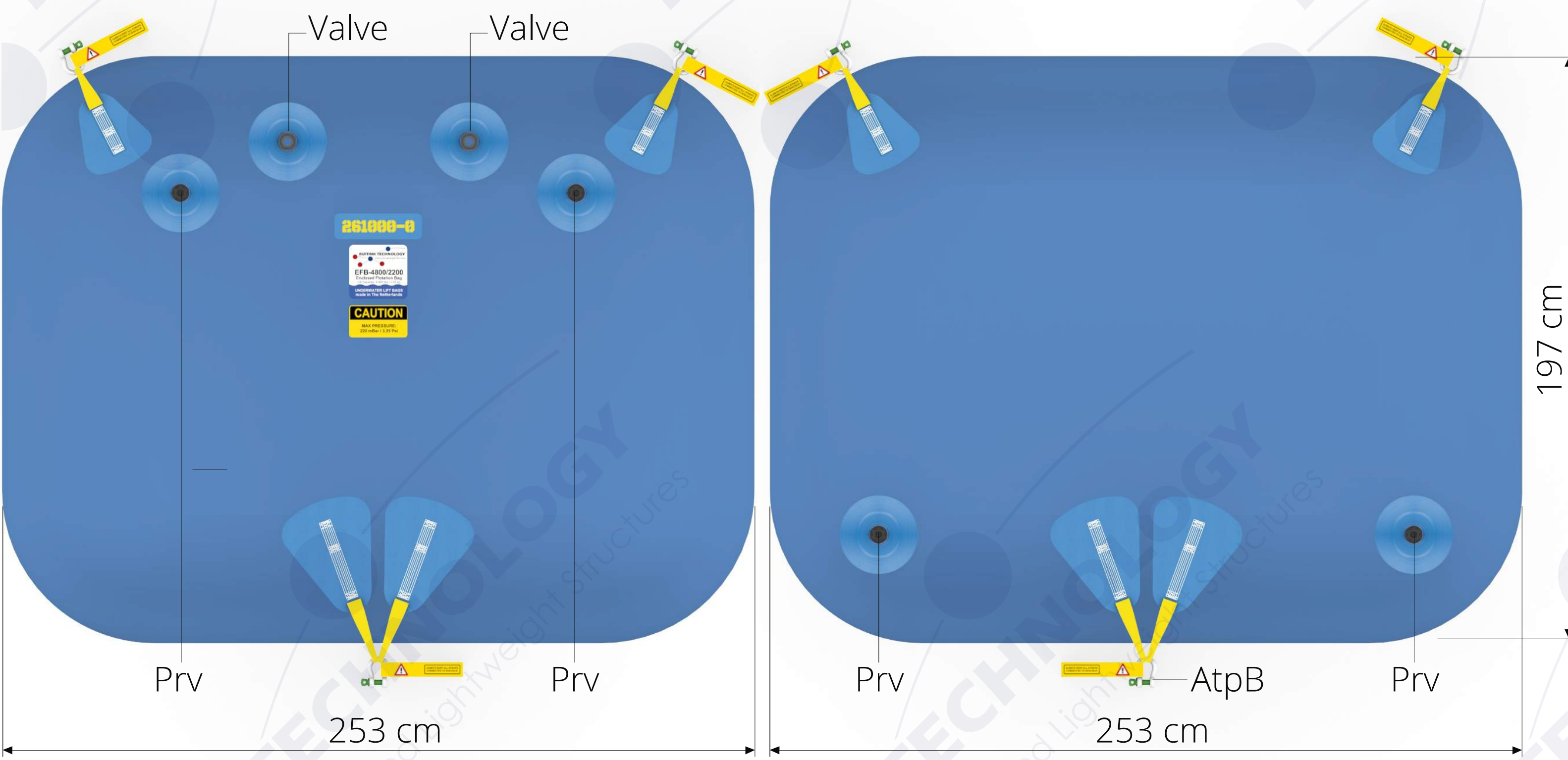
EFB-4800/2200 FRONT
