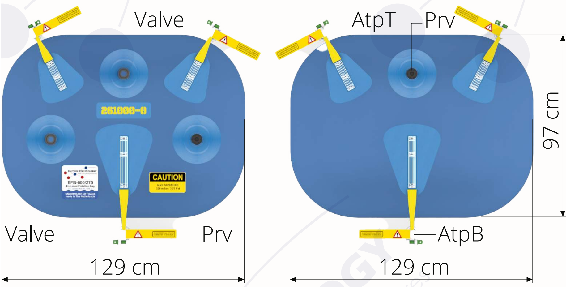
EFB-600/275 FRONT
