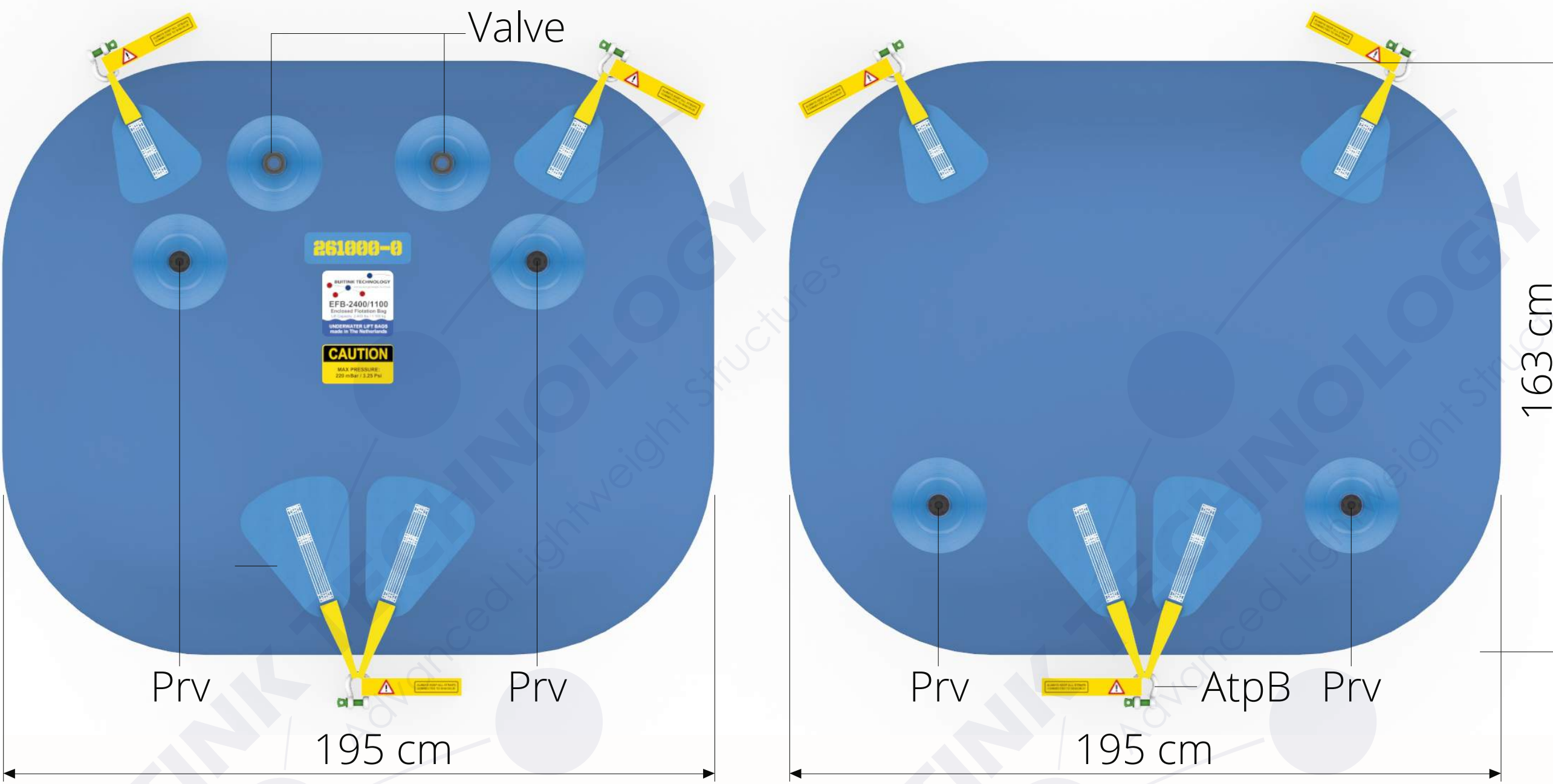
EFB-2400/1100 FRONT
